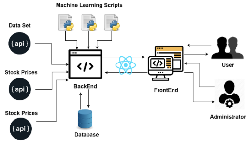
Fig. 4. System Architecture Source: Author
